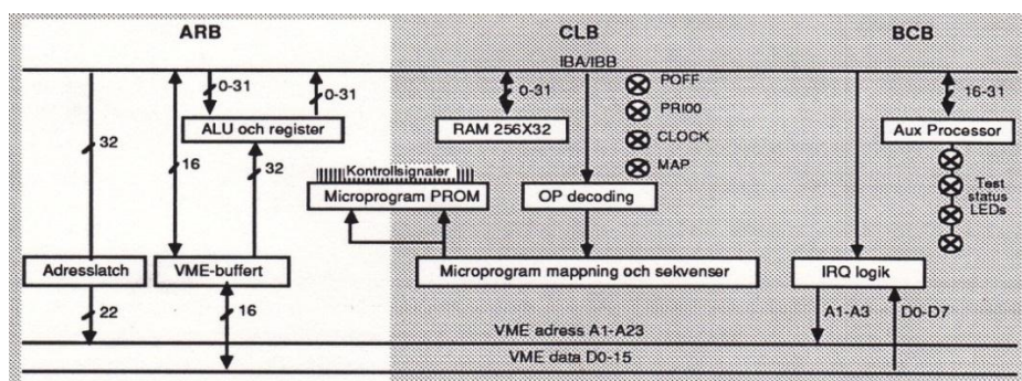
Fig. CPU 932 E blockshema
